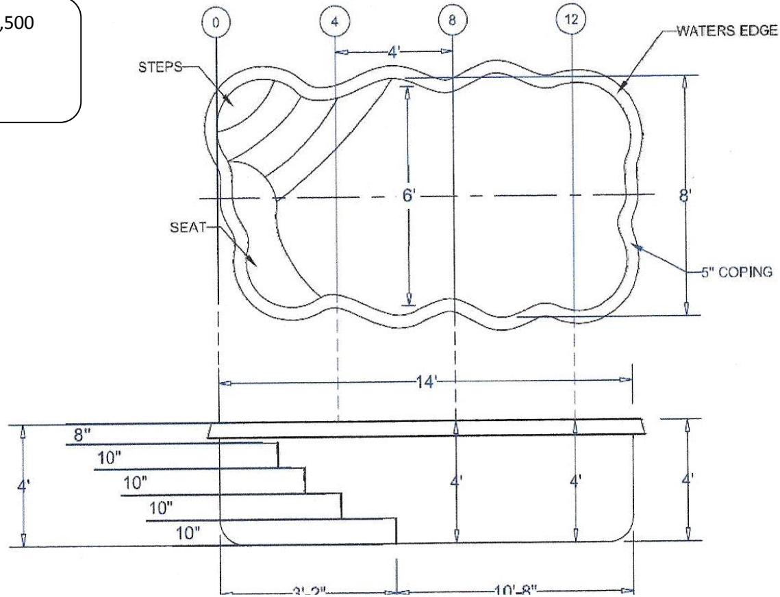
THE DENVER MODEL – 8' X 14' – 4' Flat LONESTAR FIBERGLASS POOLS
